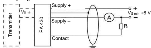
Fig. 7: Hysteresis mode
