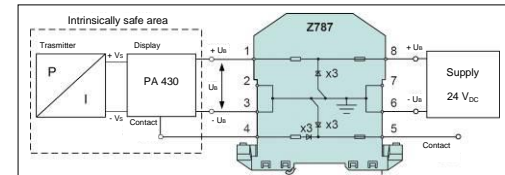
Fig. 3: circuit diagram
