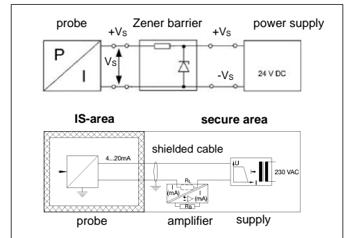
Fig. 4: Circuit diagrams
