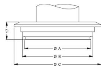
Varivent®
