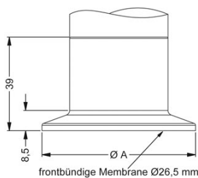
Clamp (DIN 32676)
